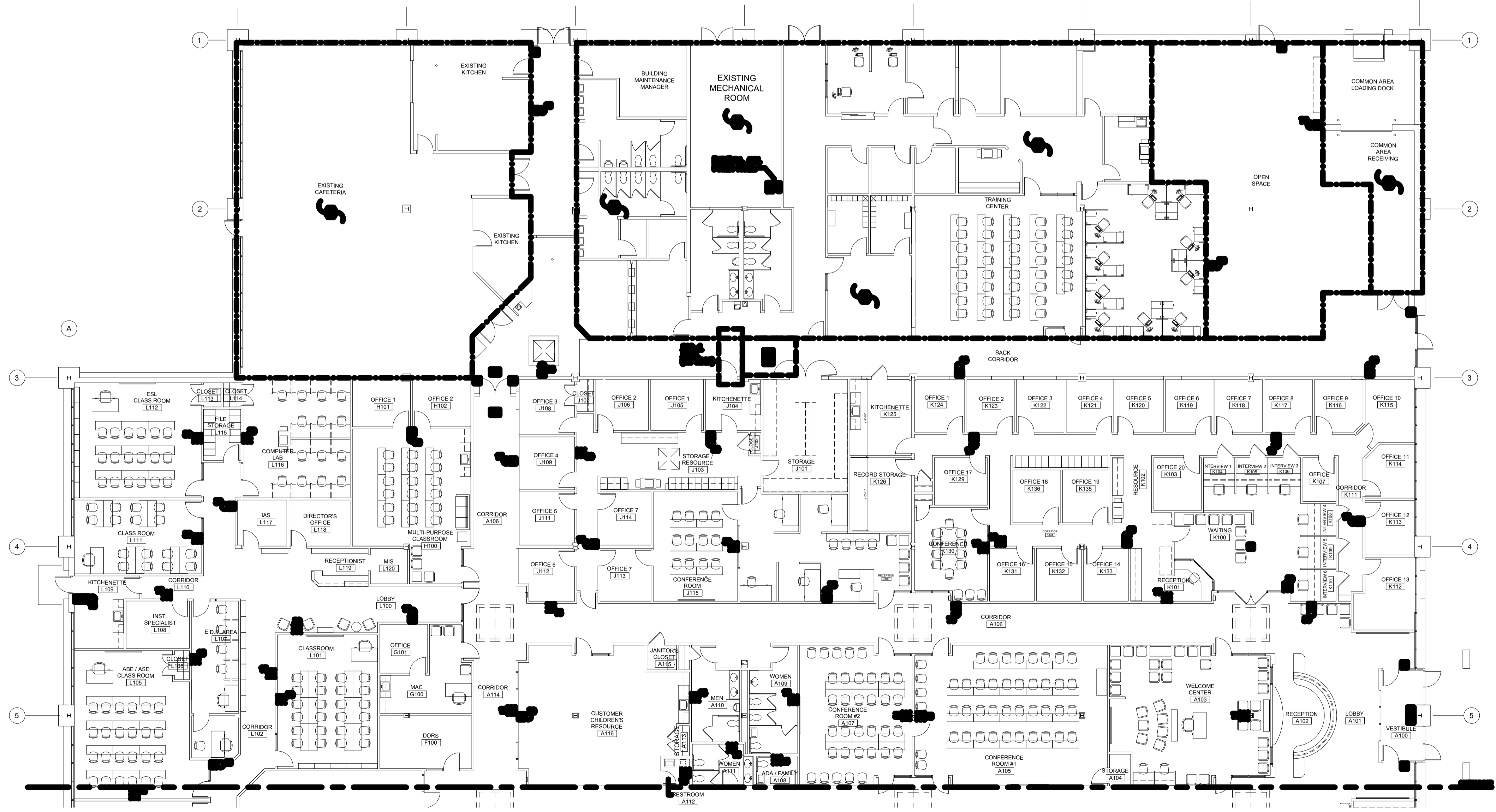
1 FIRST FLOOR PLAN - FIRE ALARM
